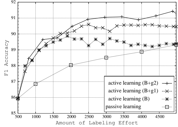
Fig. 2. Noise-robust strategies vs. baseline AL for ATIS
